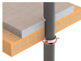
The Hilti CFS-C EL endless fire safety sleeve is the partitioning solution for wastewater applications in PVC, PP, PE, and a wide variety of sound-optimised pipes.
