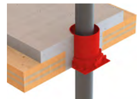
The Hilti CFS-CID cast-in element for sanitary and wastewater applications, which is cast into the XC ® slab elements at the factory, is a distinctive feature.
